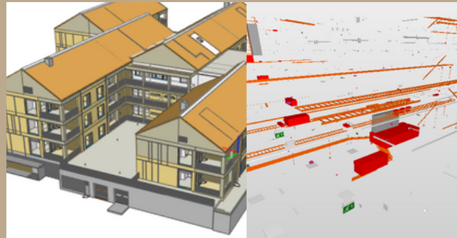
BIM Model (3D)
